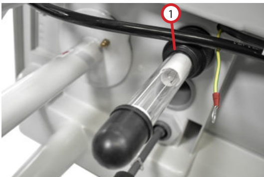
Abb. 8.1.2.6: UV-Lampe in Quarzglasröhre.
